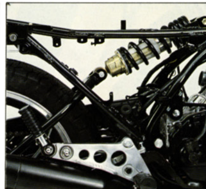
MONOCROSS SUSPENSION
